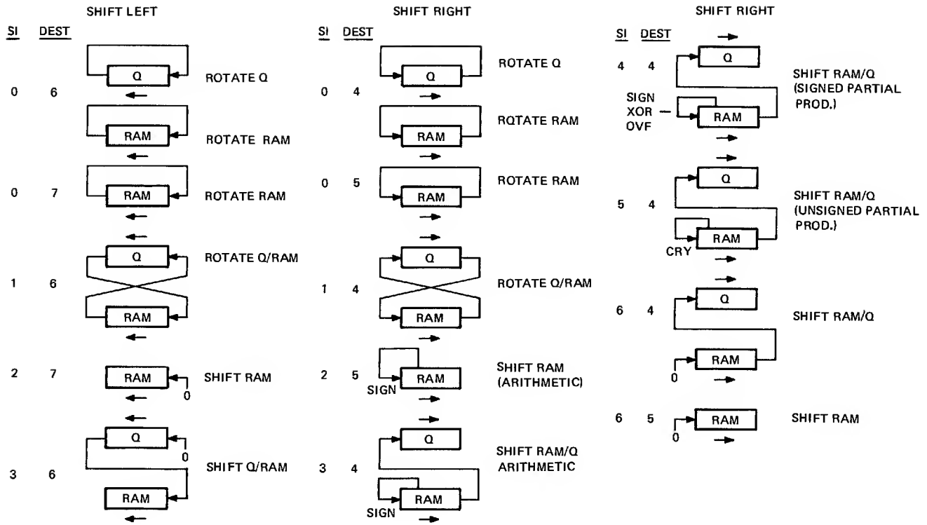
Figure 6-9 Shift Configurations
